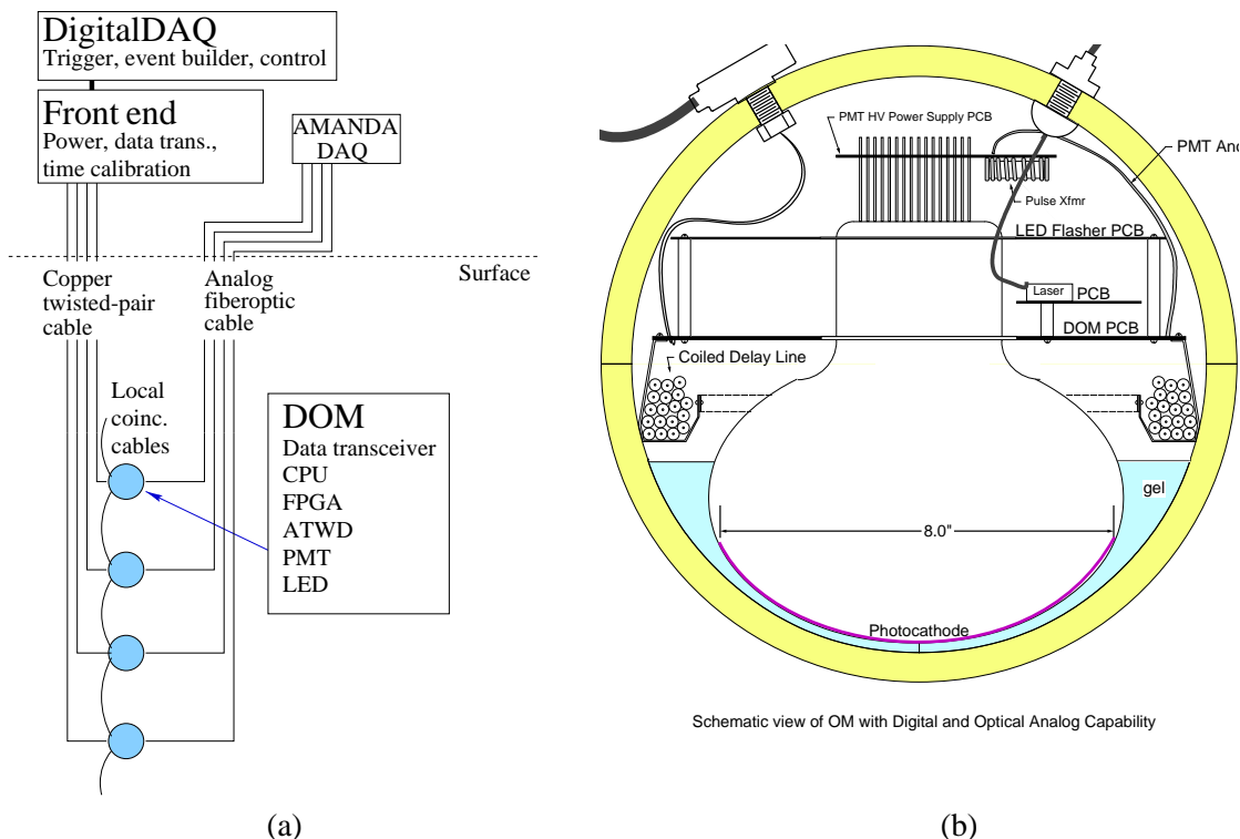
Figure 1: a. Schematic of the DOM string showing connections between the various components. b. Scale drawing of a DOM showing board placement.
