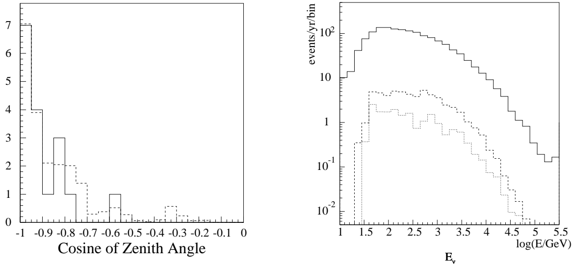
Figure 5: Left: Zenith angle distribution of neutrino candidates and of MonteCarlo simulated atmospheric neutrinos. Right: The simulated energy spectrum (true neutrino energy) is shown at trigger level of the 10 string array (solid lines), at level 3 cuts (dashed lines) and at level 4 (dotted).
