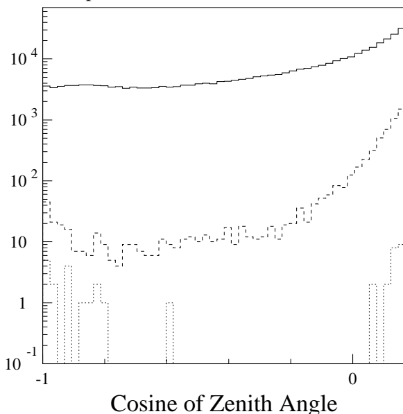
Figure 1: The reconstructed zenith angles of 85 days of AMANDA 10 string data is shown for quality level 2 (solid lines), 3 (dashed) and 4 (dotted).
