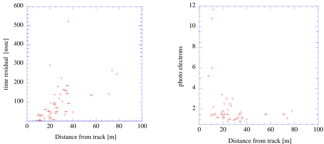
Figure 3: Event 1197960: The arrival time delay of photons with respect to the reconstructed Cherenkov cone is plotted versus the distance of the reconstructed track (left). The observed pulse amplitudes are plotted versus distance of the track (right).
