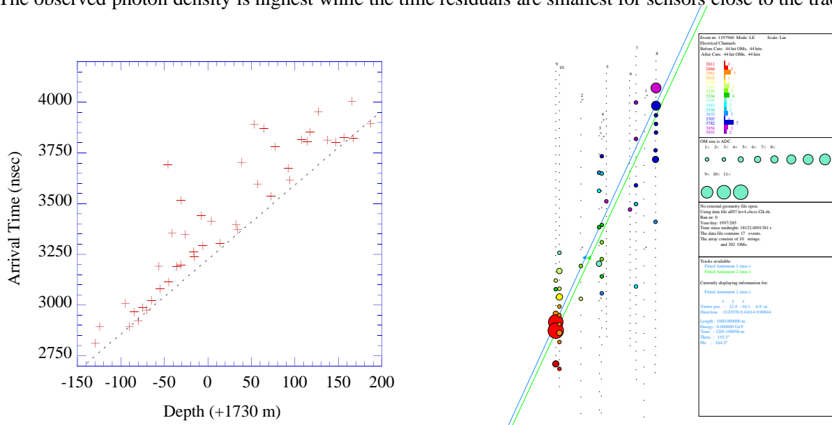
Figure 4: Event 1197960. Left: The recorded arrival times of photons are plotted versus the depth of the observing sensors. The slope of the dashed line is the result of the reconstructed zenith angle of 155^\circ . Right: Neutrino candidate event in the 10 string array. The shading (size) of the data represents time (amplitude) of triggered photomultipliers. The reconstructed muon track moves upward over more than 300 m.
